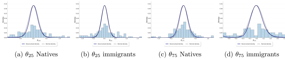
Figure G.1: Deconvolved density of immigrants' and natives' location effects
